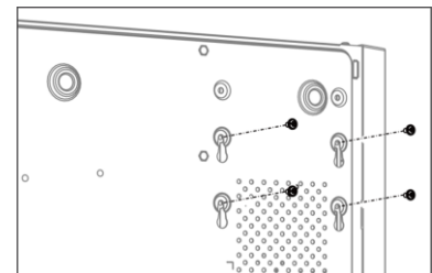
Figure 2-11 Fix HDD to Device Bottom
